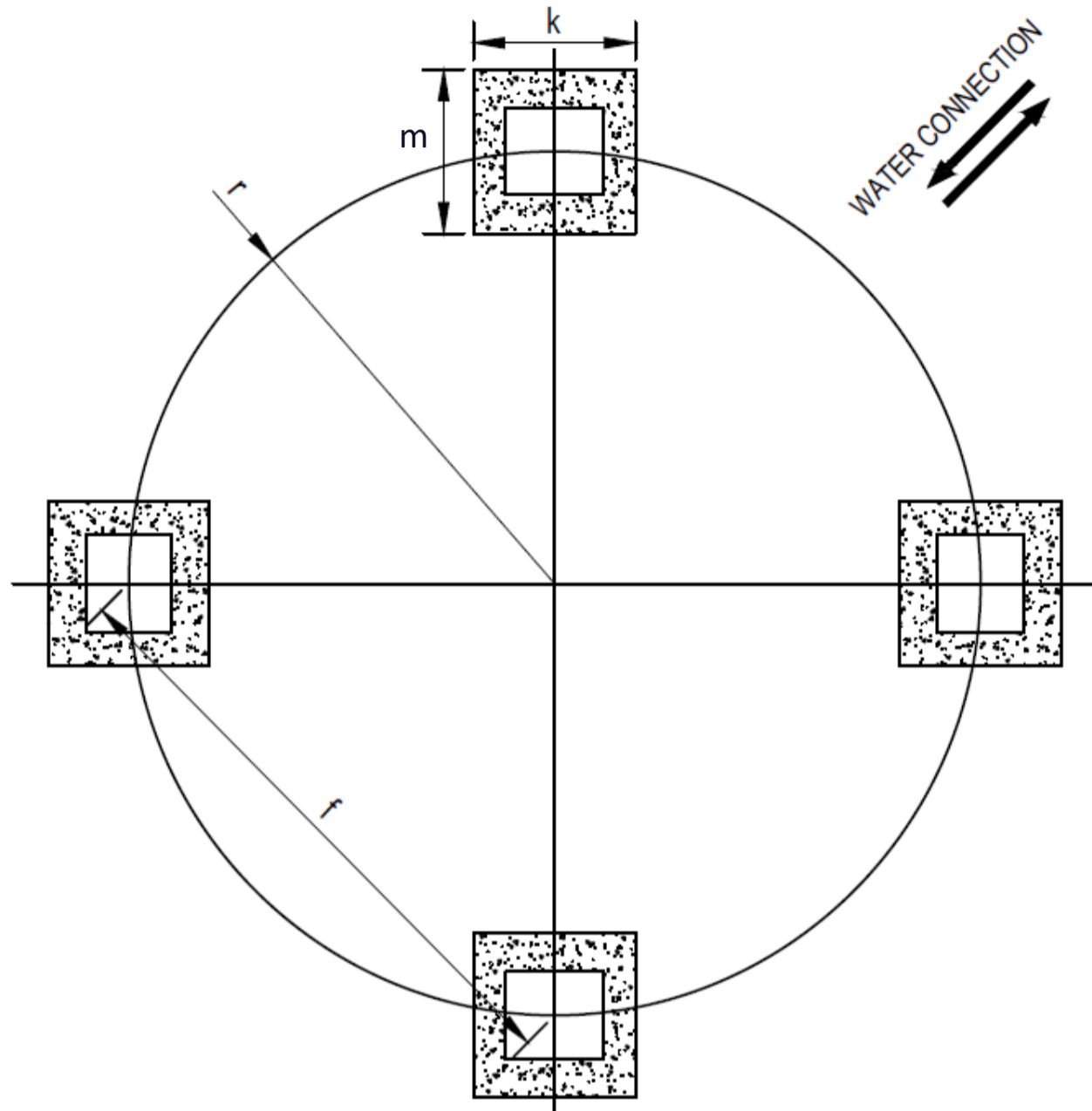
FOUNDATION DETAILS
